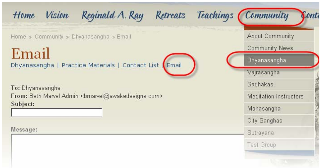
Figure 3 – Sending Email
